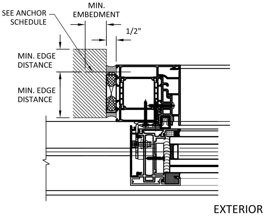
C 10 JAMB ANCHOR DETAIL
