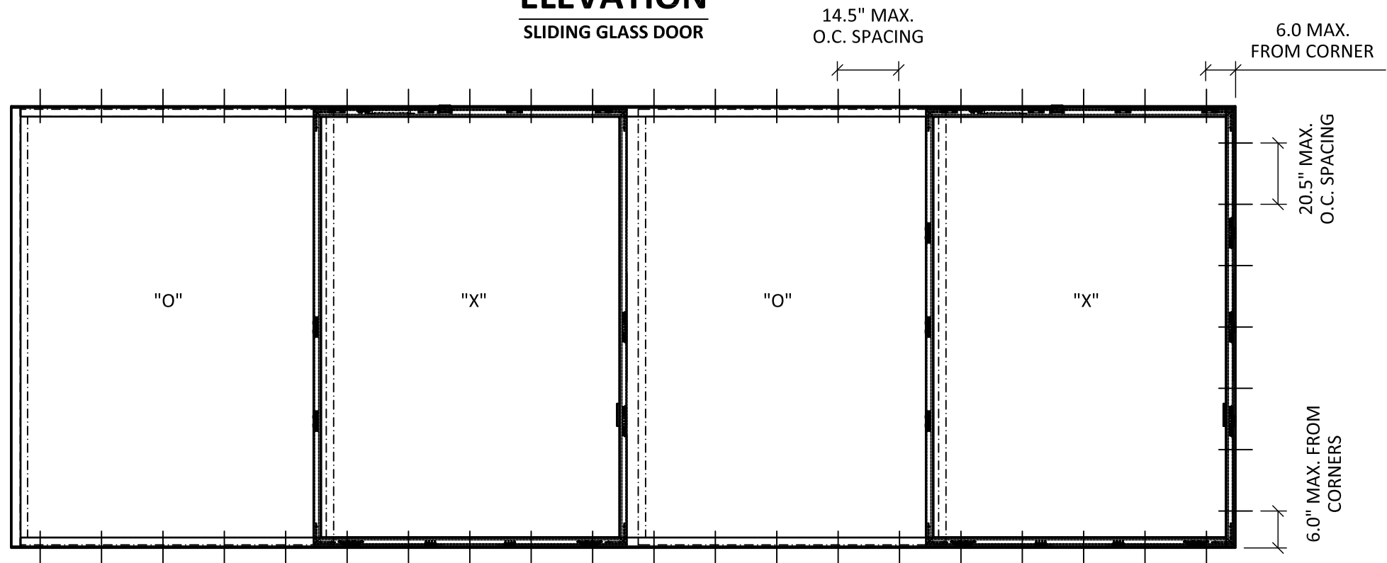
ANCHOR LAYOUT THROUGH FRAME
