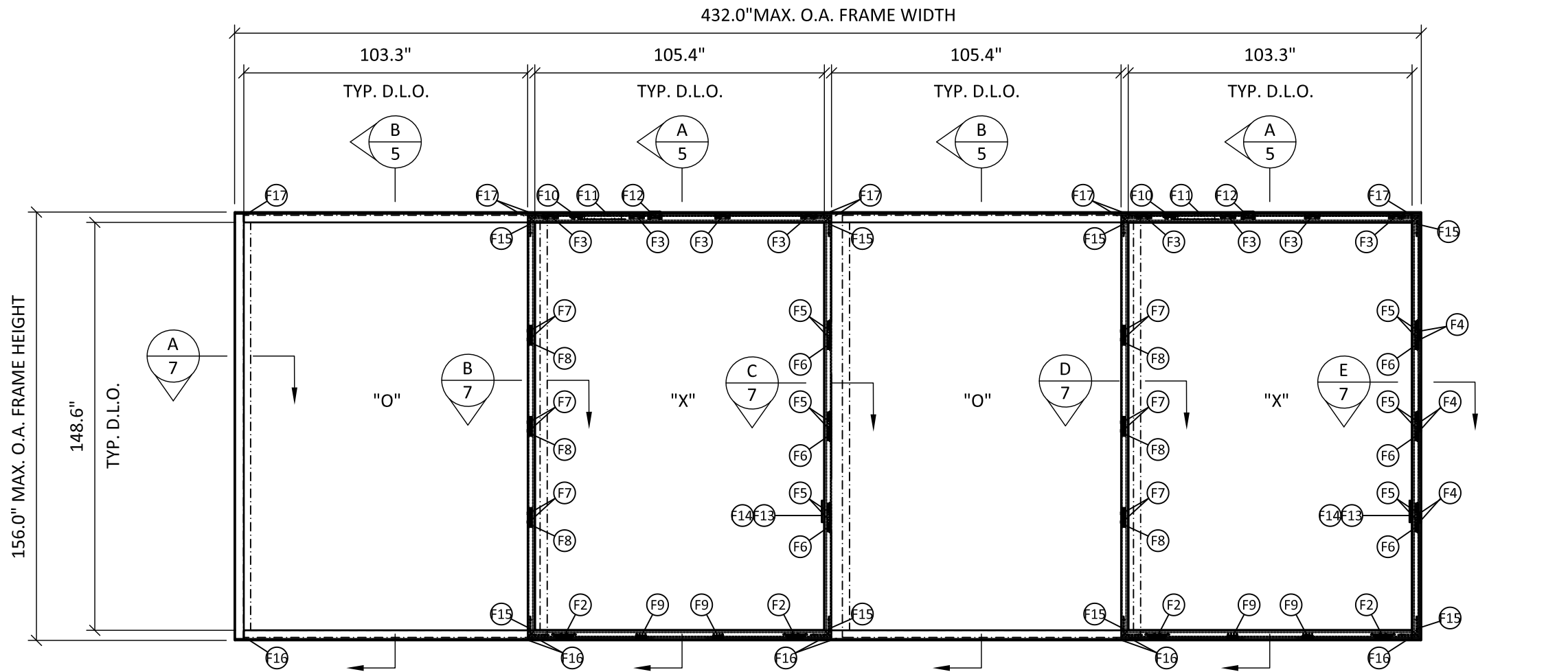
ELEVATION SLIDING GLASS DOOR
