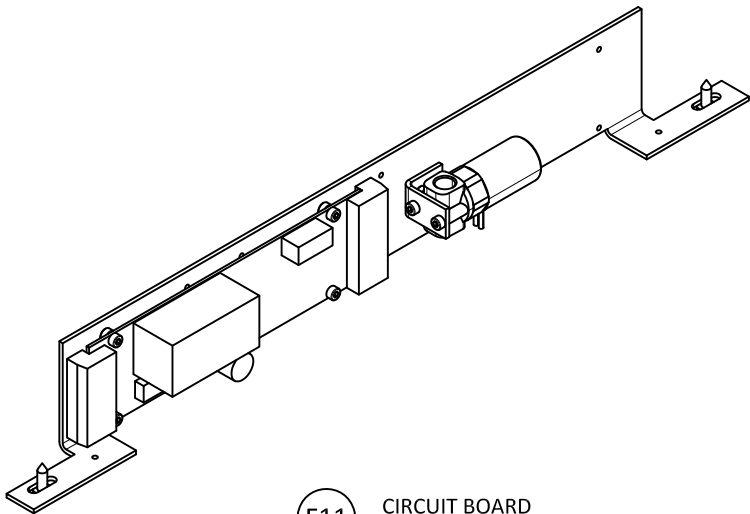
F11 CIRCUIT BOARD
