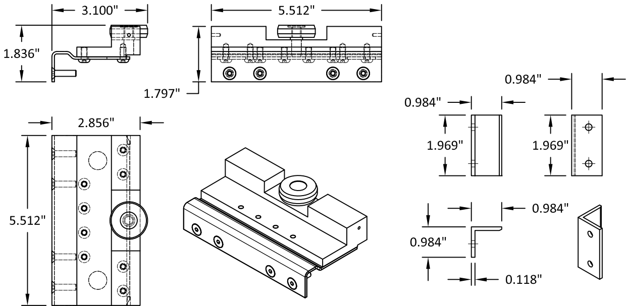
F3 LEADING ROLE
